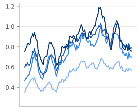
Spread / RMSE
