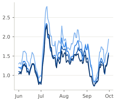
NeuralGCM
