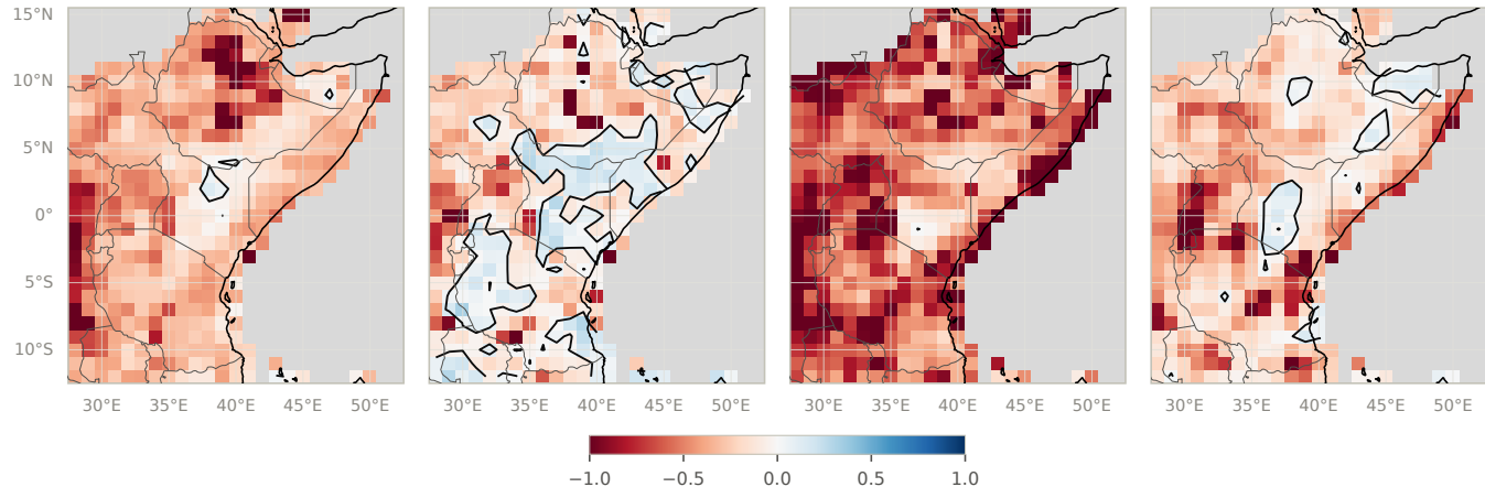
Skill vs climatology by model, lead day 1, MAM 2024 (CHIRPS) FourCastNet GenCast GraphCast NeuralGCM
