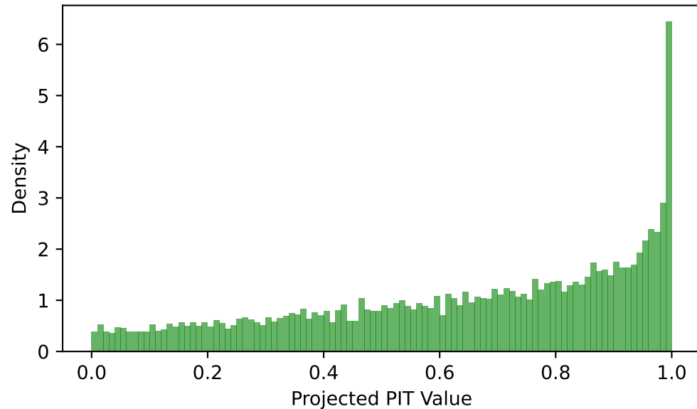
PIT - Projection 1
