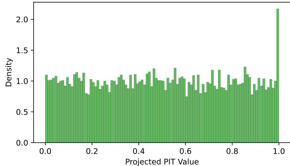
PIT - Projection 1
