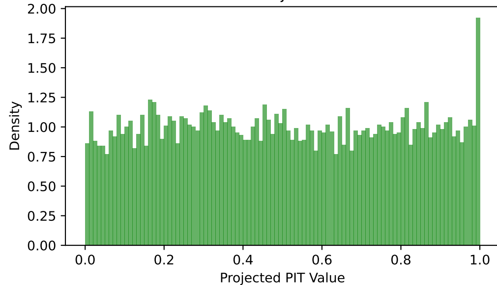
PIT - Projection 1
