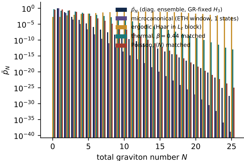
late-time multiplicity, \tilde{g} = 12 , d = 6 , L_z = 0
