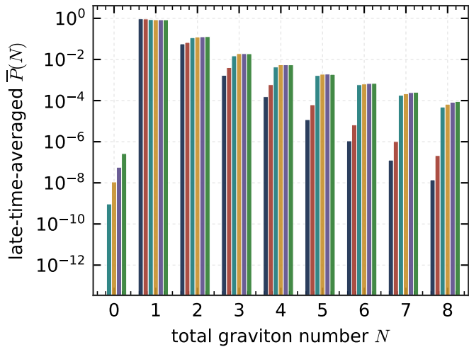
(b) multiplicity tower
