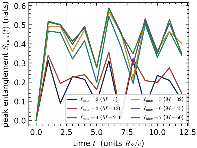
(a) peak-entanglement dynamics
