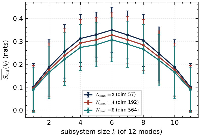
multi- \ell profile ( \ell = 2 \oplus 3 , t = 20 , L_z = 0 )
