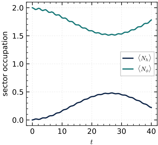
cascade populations, \tilde{g}_3 = 12 , \tilde{g}_m = 12
