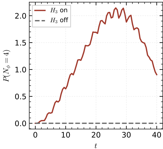
four-scalar yield: the new channel 1e-5
