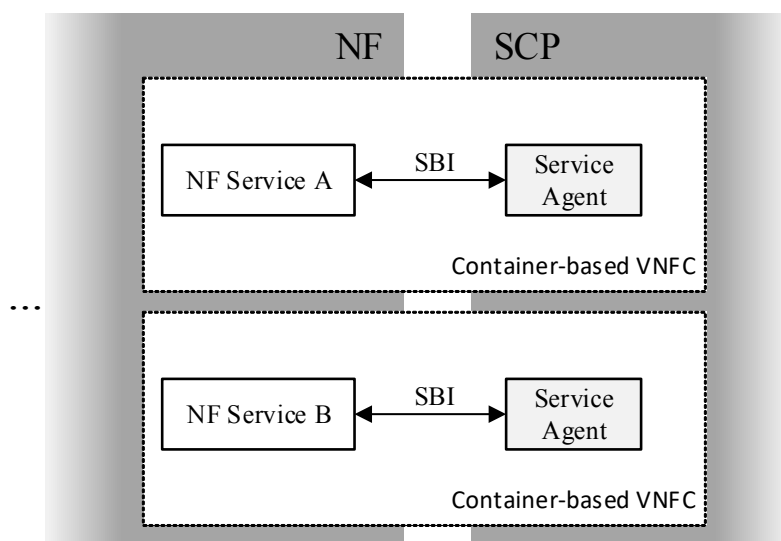
Figure G.2.1-3: Detail of the NF-SCP boundary
