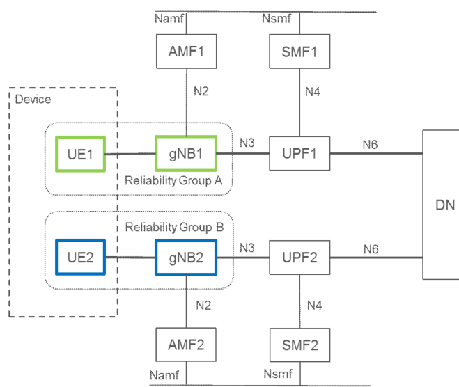
Figure F-2: Reliability group-based redundancy concept in RAN
