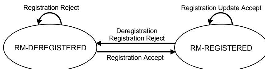
Figure 5.3.2.4-1: RM state model in UE
