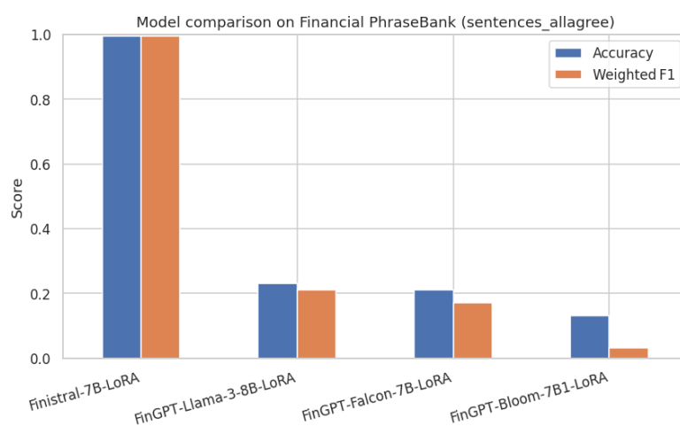
Fig. 5: Finistral-7B-LoRA vs FinGPT Baseline LoRA on Financial PhraseBank
