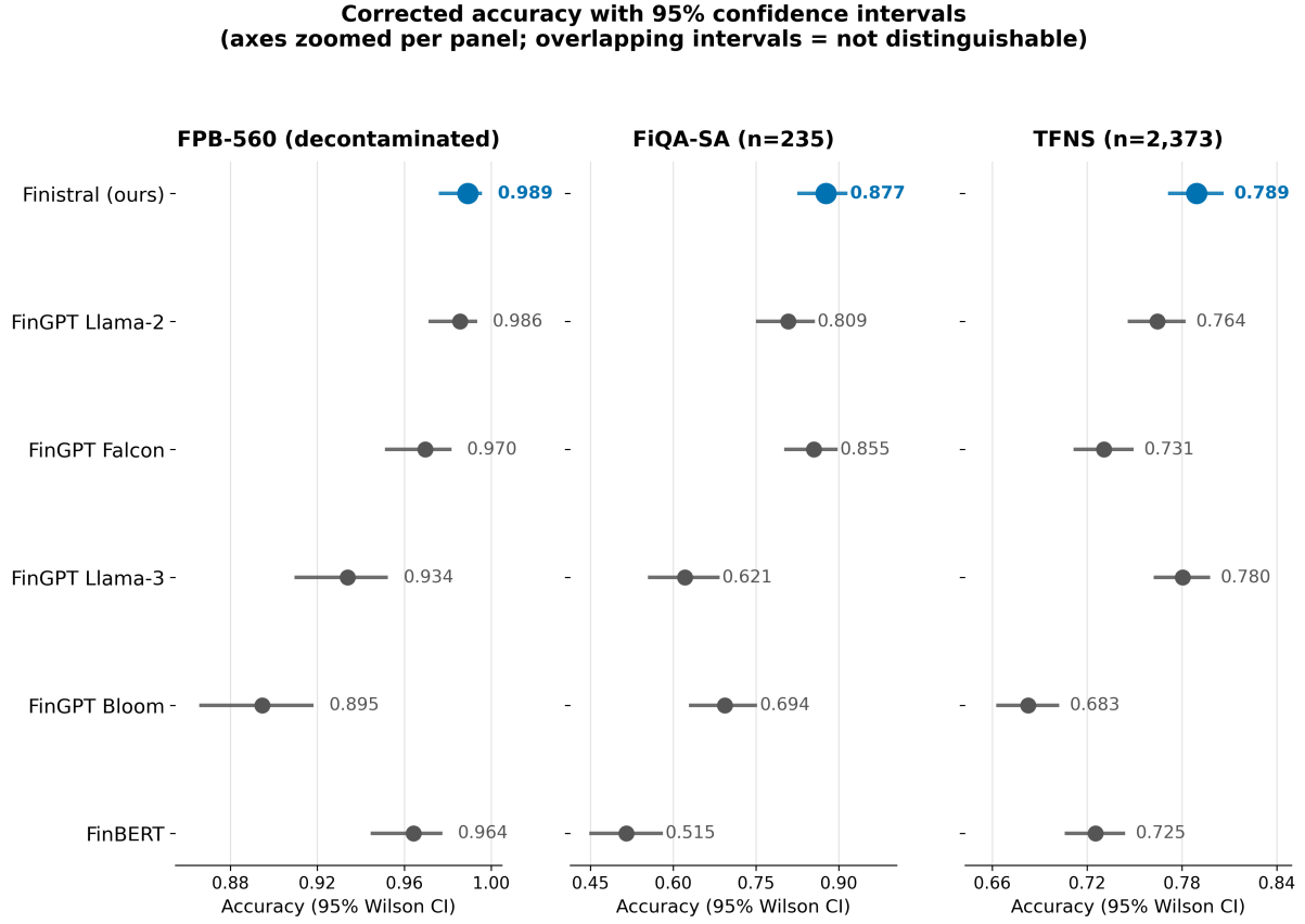
Fig. 4: Corrected accuracy of Finistral-7B-LoRA against all FinGPT adapter baselines and FinBERT on the exact-match-decontaminated sets, with 95% Wilson confidence intervals. Axes are zoomed per panel to resolve small differences; because value is encoded by position rather than bar length, the non-zero origin introduces no visual exaggeration. Overlapping intervals indicate differences that are not statistically distinguishable — note the overlap with FinGPT-mt-Llama2 on FPB-560, FinGPT-Falcon on FiQA-SA, and FinGPT-Llama-3 on TFNS, matching the McNemar results in Appendix A. Weighted and macro F1 for every model are given in Table 8 and Appendix A; the unparsable-dominated zero-shot backbone is omitted here and shown in Figure 3.
