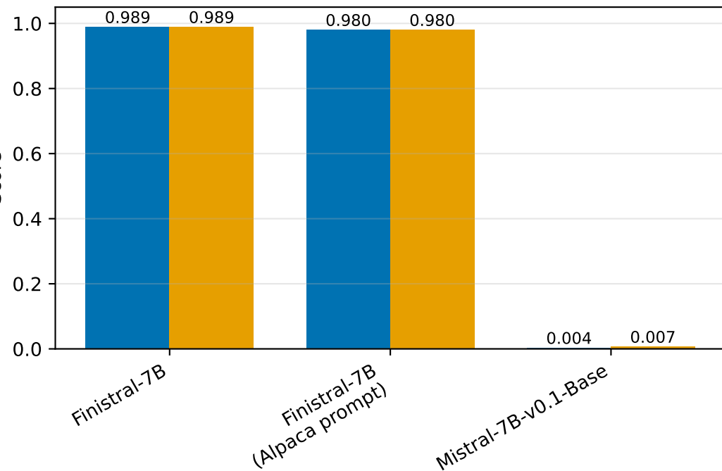
FPB decontaminated (n=560)
