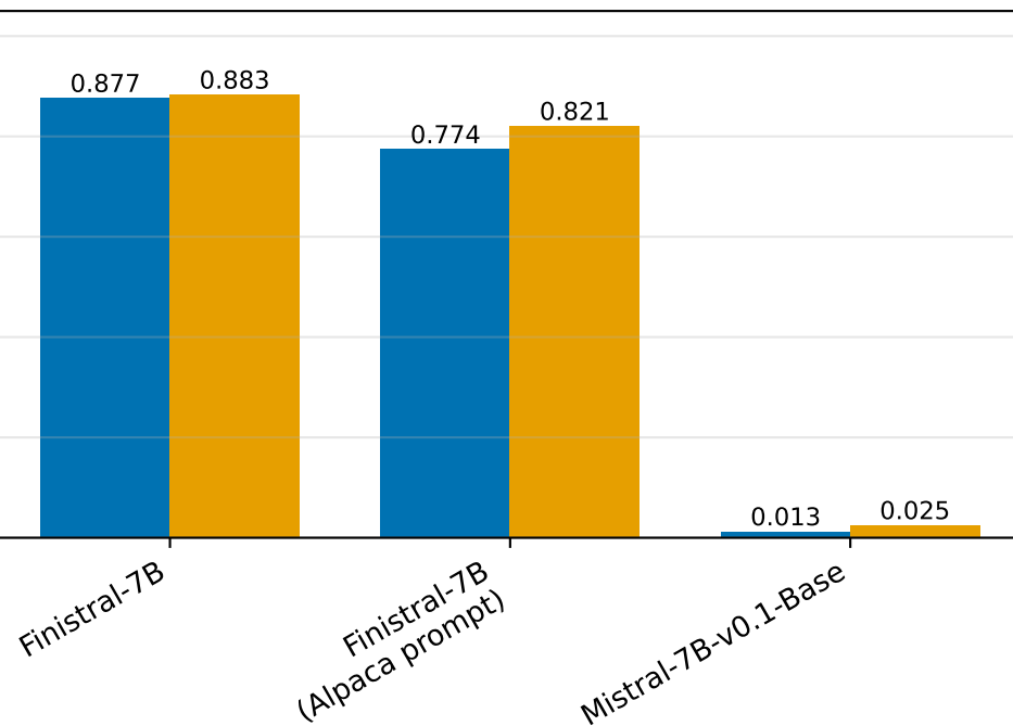
FiQA-SA (decontaminated, n=235)
