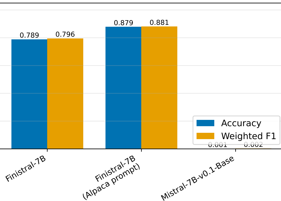
TFNS (decontaminated, n=2,373)
