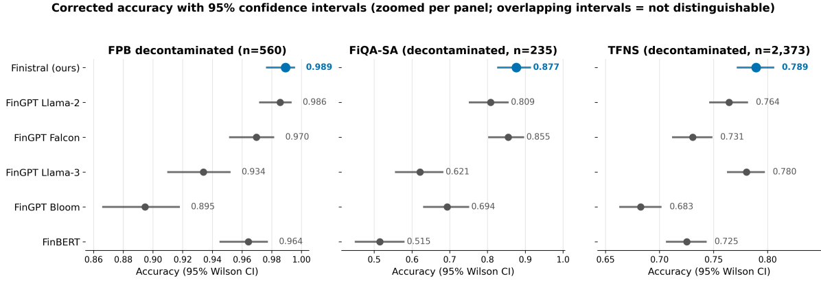
Fig. 4: Corrected accuracy of Finistral-7B-LoRA against all FinGPT adapter baselines and FinBERT on the exact-match-decontaminated sets, with 95% Wilson confidence intervals. Axes are zoomed per panel to resolve small differences; because value is encoded by position rather than bar length, the non-zero origin introduces no visual exaggeration. Overlapping intervals indicate differences that are not statistically distinguishable — note the overlap with FinGPT-mt-Llama2 on FPB-560, FinGPT-Falcon on FiQA-SA, and FinGPT-Llama-3 on TFNS, matching the McNemar results in Appendix A. Weighted and macro F1 for every model are given in Table 8 and Appendix A; the unparseable-dominated zero-shot backbone is omitted here and shown in Figure 3.
