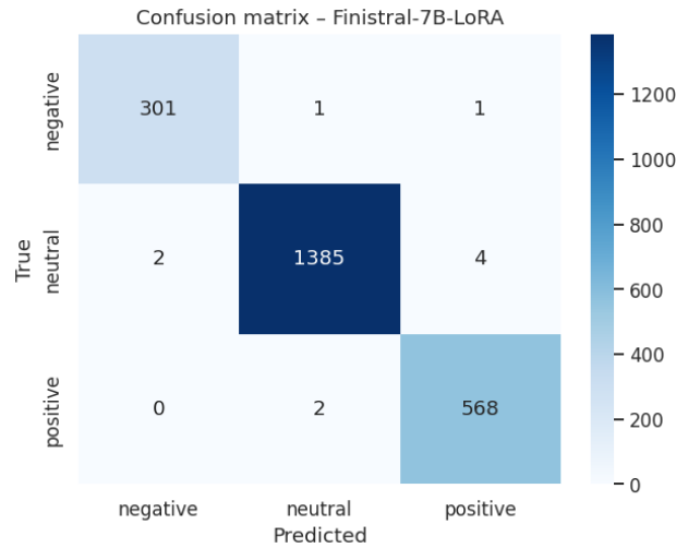
Fig. 5: Confusion matrix of Finistral-7B-LoRA on the original, contaminated full split, retained solely as a contamination diagnostic (Section 5.5); the corrected per-model confusion matrices appear in Figure 6.
