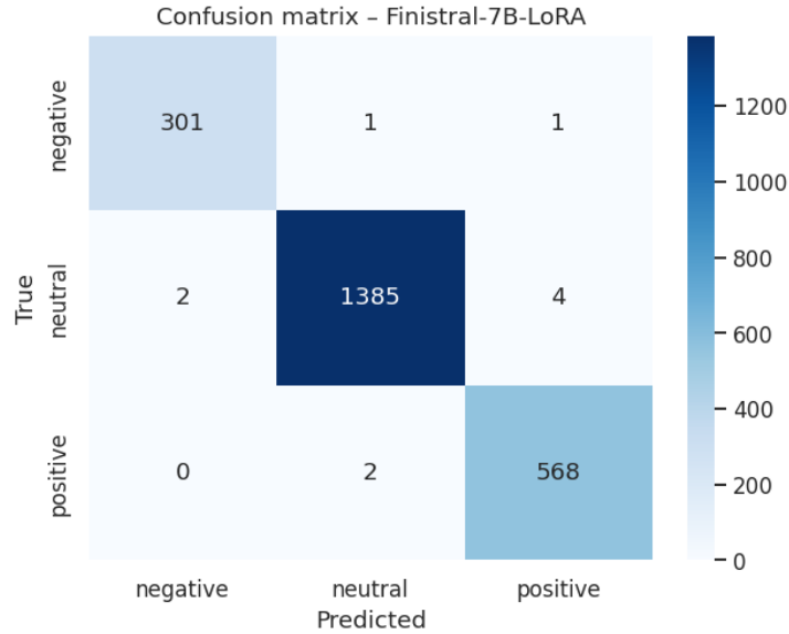
Fig. 6: Confusion matrix – Finistral-7B-LoRA
