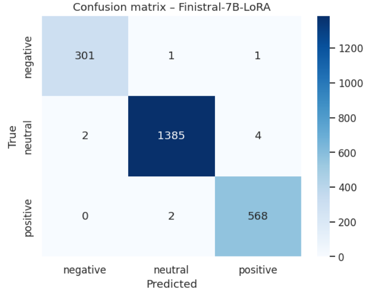
Fig. 6: Confusion matrix – Finistral-7B-LoRA
