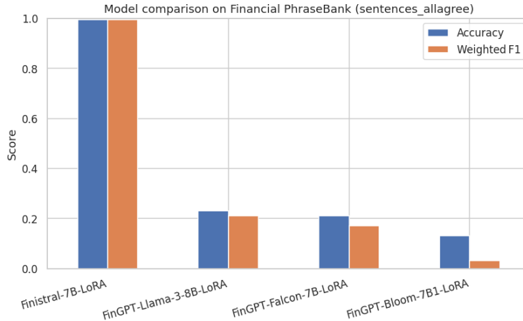
Fig. 5: Finistral-7B-LoRA vs FinGPT Baseline LoRA on Financial PhraseBank
