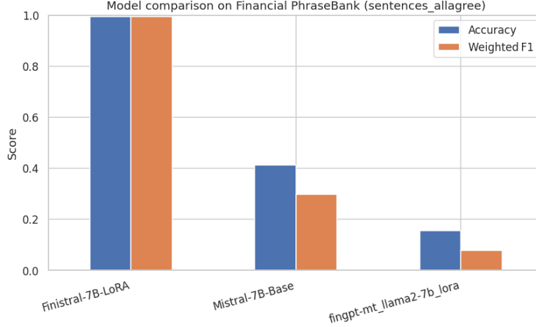
Fig. 4: Finistral-7B-LoRA vs Mistral-7B-Base on Financial PhraseBank (sentences_allagree)
