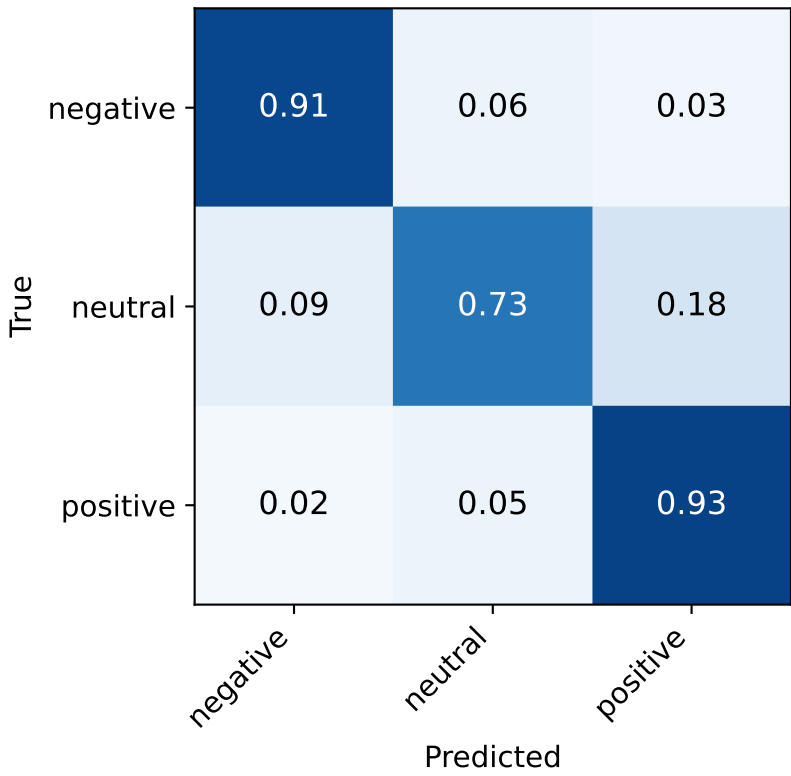
Mistral-7B-v0.1-Base
