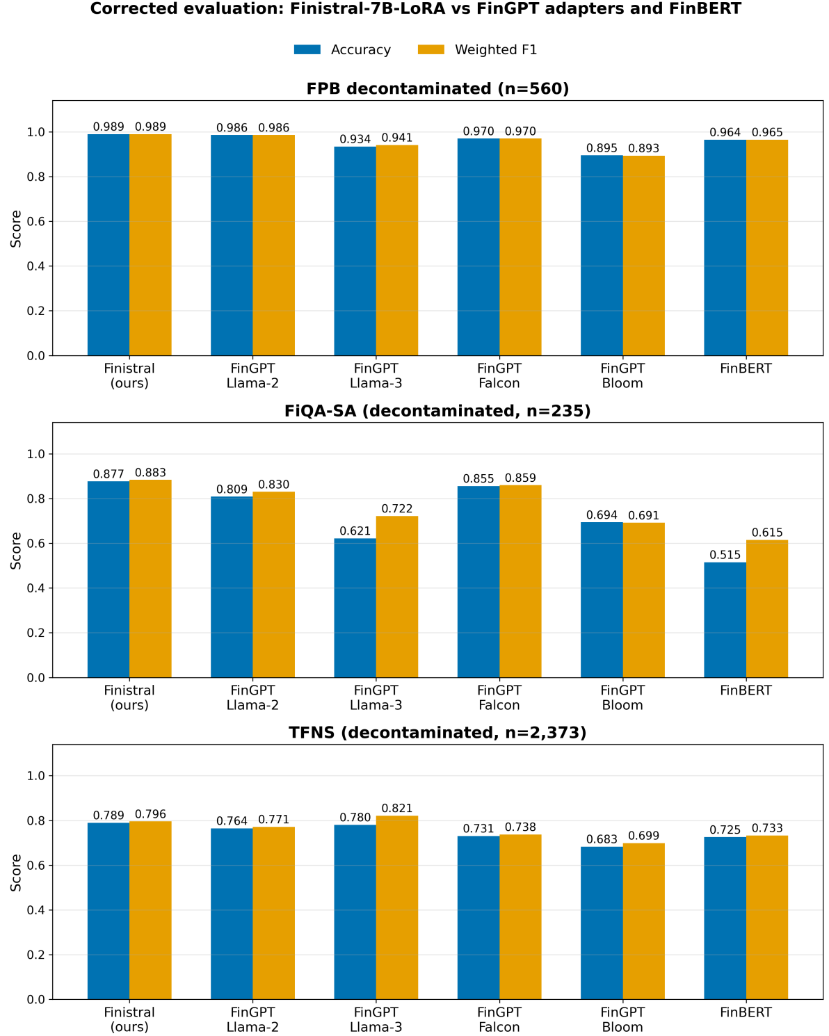
Fig. 4: Corrected comparison (exact-match-decontaminated sets) of Finistral-7B-LoRA against all FinGPT adapter baselines and FinBERT, per evaluation set. Missing bars indicate accuracy/F1 near zero (the unparseable-dominated zero-shot backbone is omitted; see Table 8).
