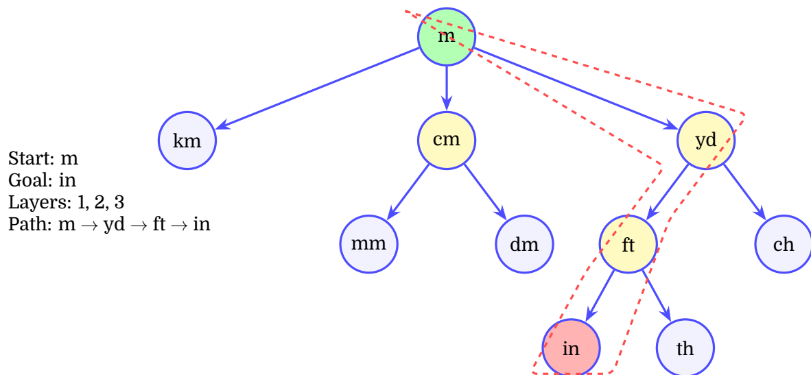
Figure 3.1: BFS exploration tree. Green node is start, yellow nodes explored before red goal node (in). Dashed red line shows shortest path found. All unit nodes are circles.
