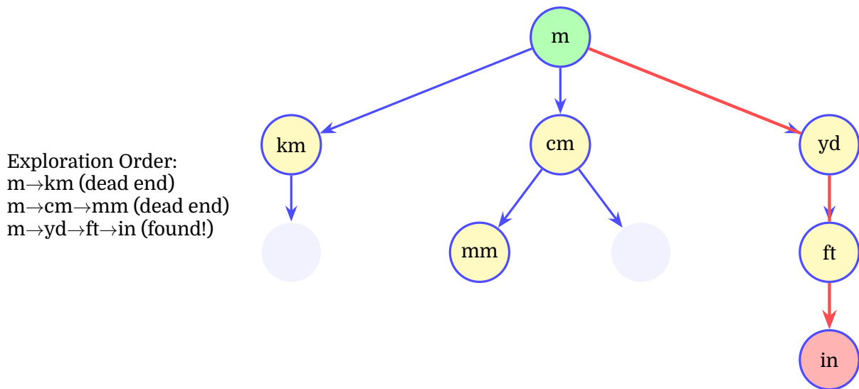
Figure 3.2: DFS exploration tree. Thick red arrows show the path DFS follows. Yellow nodes explored before finding goal. All unit nodes are circles.
