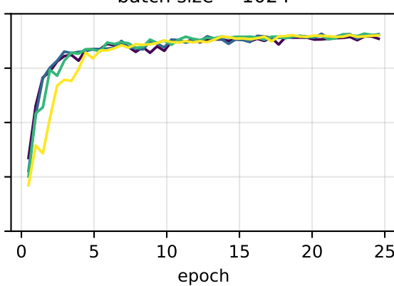
batch size = 1024
