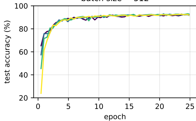
batch size = 512
