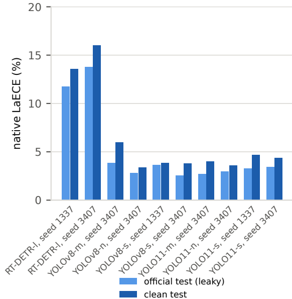
b. Calibration on D-Fire test
