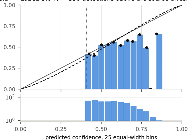
b. YOLOv8-s → Pyro-SDIS (shifted)
