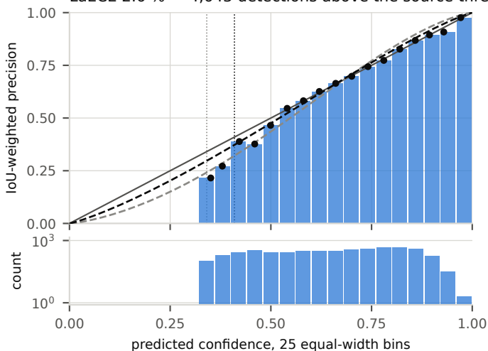
a. YOLOv8-s → D-Fire test (in-domain)
