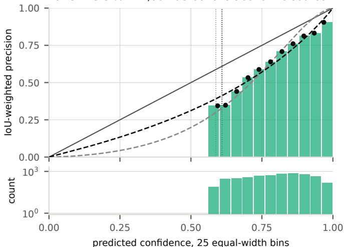
c. RT-DETR-L → D-Fire test (in-domain)
