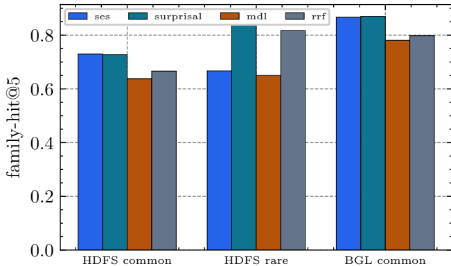
Failure-family retrieval by scorer (v4 semantics)
