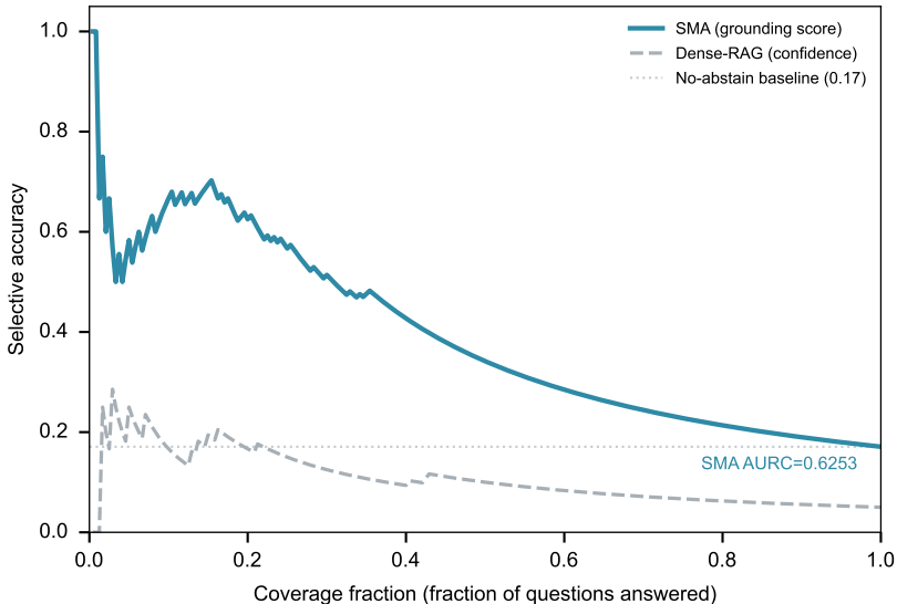
ED Phase 5 risk-coverage (selective prediction)
