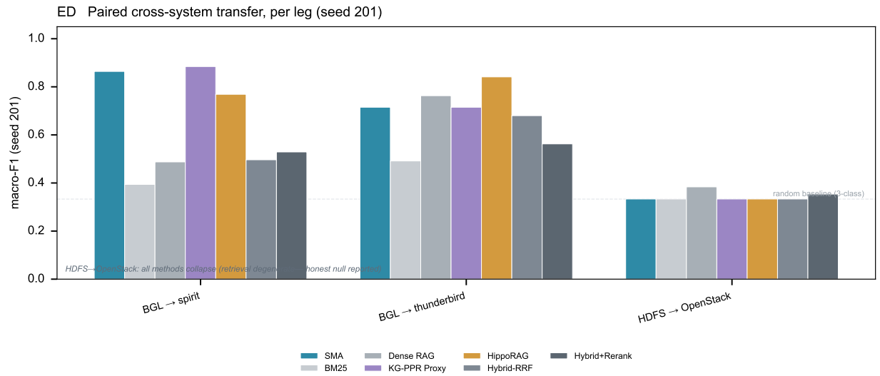
Extended Data Fig. 3 | Paired cross-system transfer, per leg (seed 201). macro-F1 for each transfer leg of the LogHub benchmark ( t1_transfer_metrics.csv ), comparing SMA against all base-lines without leg-averaging (which masks per-leg imbalance). BGL → Thunderbird: SMA achieves 0.715 macro-F1. BGL → Spirit: SMA is competitive but one seed shows large variance (seeds 201–205 are shown in aggregate stats in t1_stats.csv ). HDFS → OpenStack: all methods collapse to 0.333 (retrieval degeneracy; three-class uniform prediction; documented diagnostic in the CSV). The honest null on HDFS → OpenStack is reported and does not affect the main claims. Source: reports/confirmatory/t1_transfer_metrics.csv .
