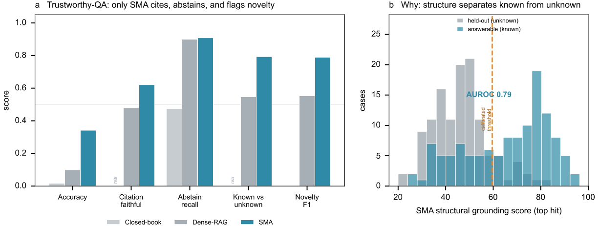
Figure 3: The SMA-grounded LLM agent is a verifiable specialist (medicine; n=120 answerable + 120 held-out; language model and prompt fixed, memory swapped). (a) Trustworthy-QA axes for closed-book / dense-RAG / SMA: accuracy, citation-faithfulness, abstain-recall, known-versus-unknown discrimination (grounding AUROC), and novelty F1; closed-book has no retrieval, so its citation and grounding cells are N/A (marked), not zero. (b) Mechanism: SMA’s raw structural grounding score (top hit) separates answerable (known) from held-out (unknown) cases, AUROC 0.79; the dashed line is the cite-or-abstain threshold calibrated on a disjoint split. Dense cosine similarity barely separates the two (AUROC 0.55), forcing its gate to over-abstain.
