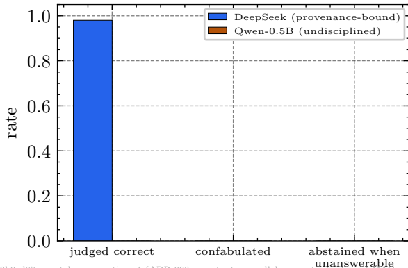
H3: judged honesty across 200 answer cells
