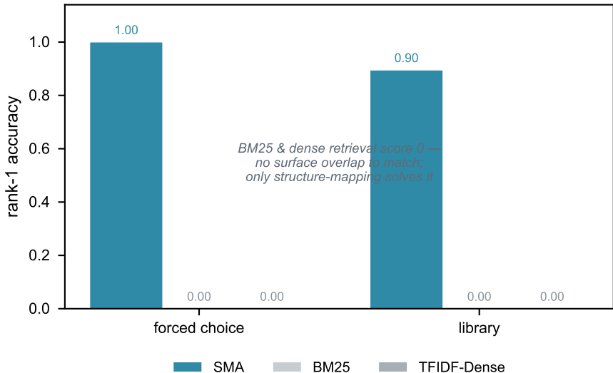
SSB: only structure survives a zero-lexical-overlap gap
