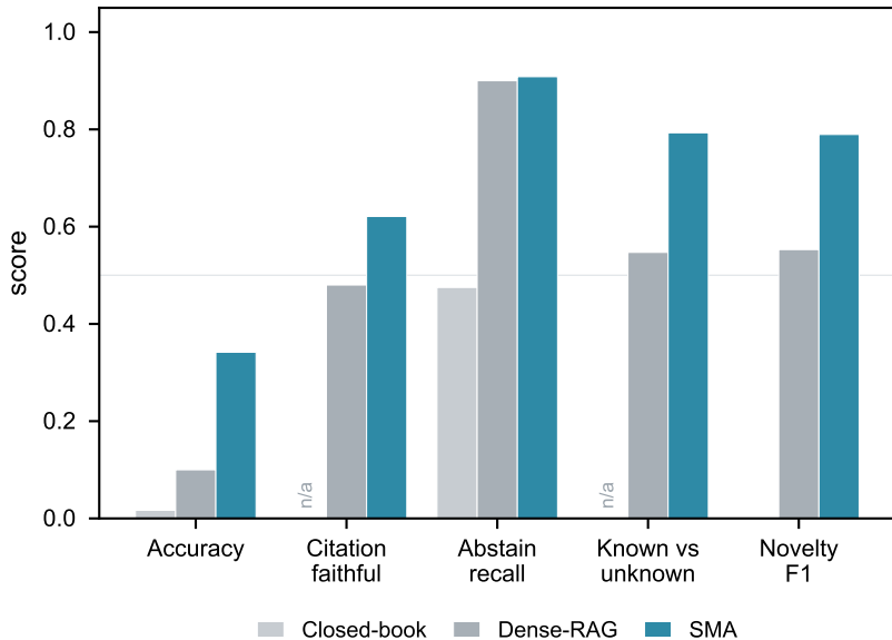
a Trustworthy-QA across memories
