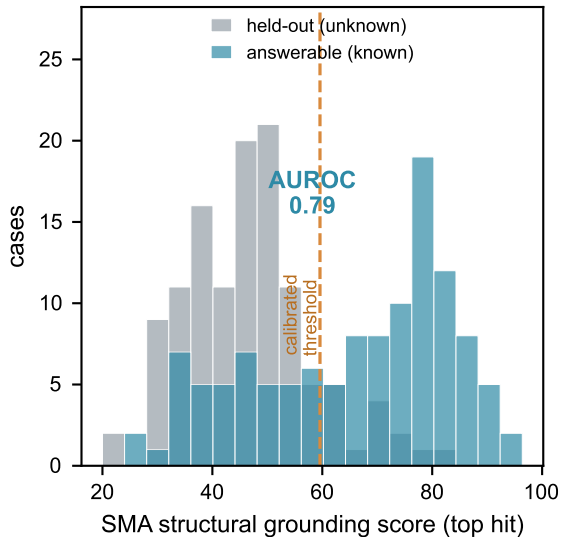
b Structure separates known from unknown
