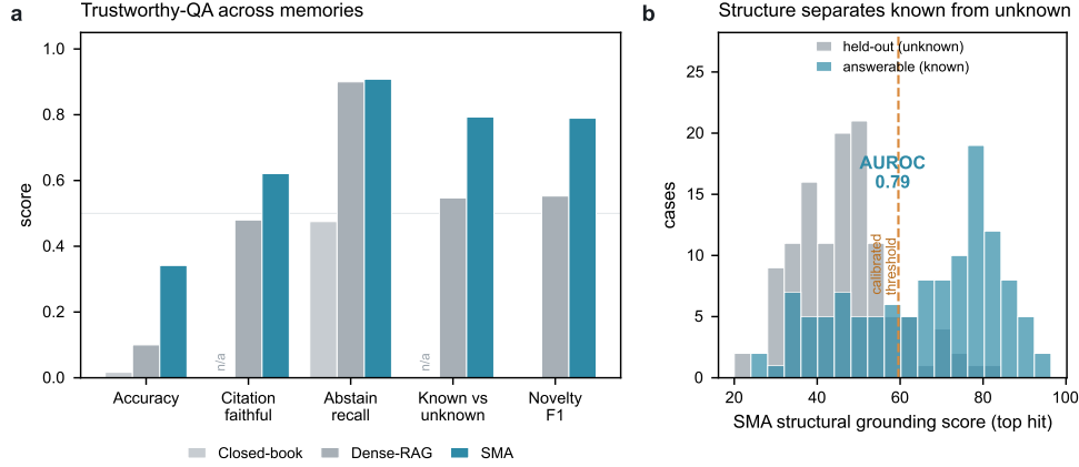
Fig. 3 The SMA-grounded LLM agent is a verifiable specialist (medicine; n=120 answerable + 120 held-out; language model and prompt fixed, memory swapped). (a) Trustworthy-QA axes for closed-book / dense-RAG / SMA: accuracy, citation-faithfulness, abstain-recall, known-versus-unknown discrimination (grounding AUROC), and novelty F1; closed-book has no retrieval, so its citation and grounding cells are N/A (marked), not zero. (b) Mechanism: SMA’s raw structural grounding score (top hit) separates answerable (known) from held-out (unknown) cases, AUROC 0.79; the dashed line is the cite-or-abstain threshold calibrated on a disjoint split. Dense cosine similarity barely separates the two (AUROC 0.55), forcing its gate to over-abstain.
