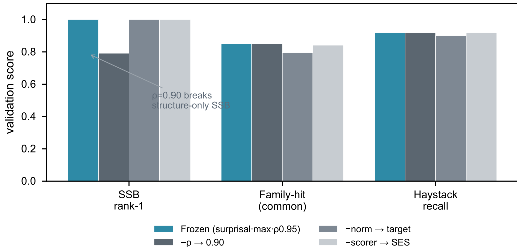
Frozen dials win the calibration grid
