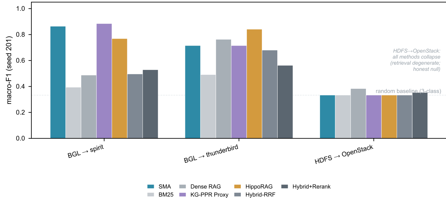
Paired cross-system transfer, per leg (seed 201)
