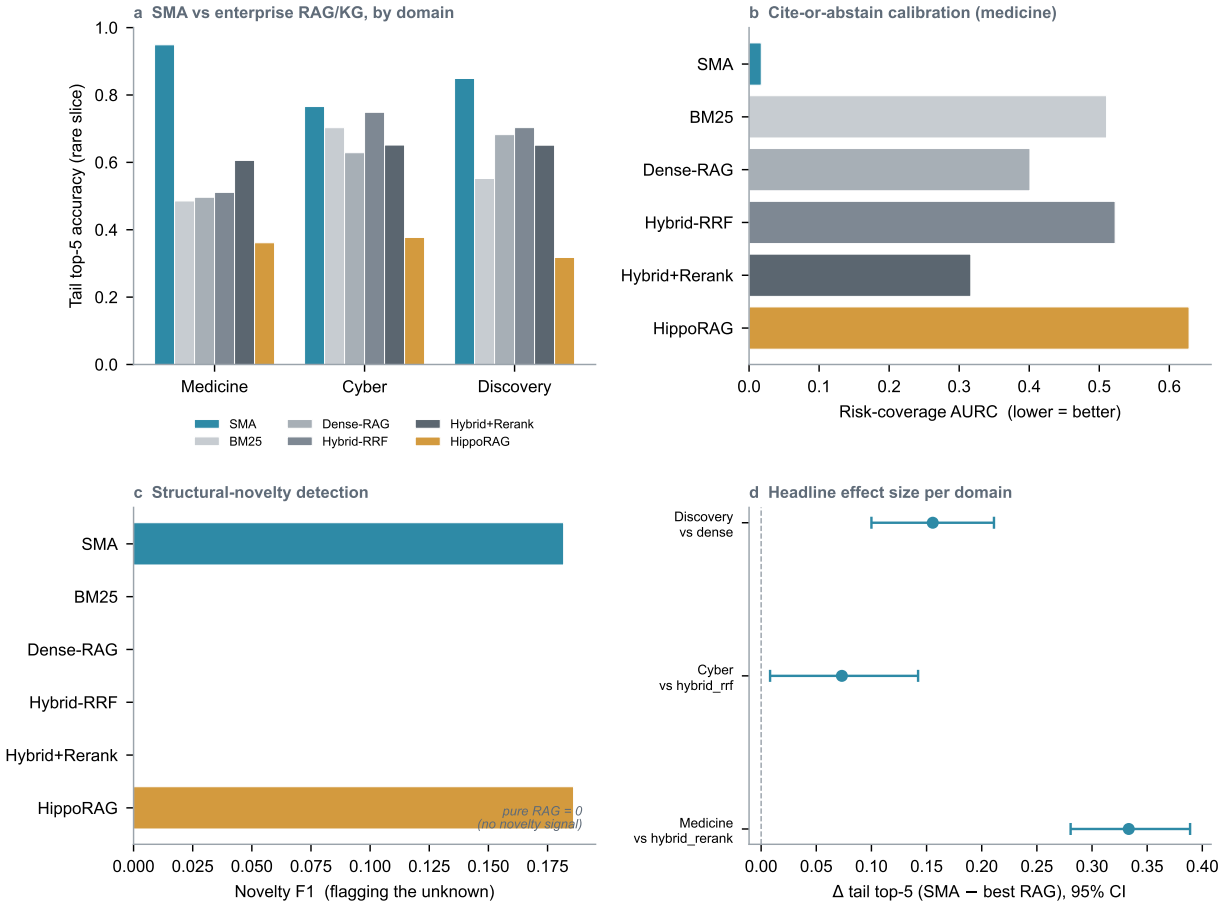
Figure 2: Agentic memory-swap results. (a) Tail top-5 (rare slice) by domain: SMA versus the enterprise RAG/KG gauntlet. (b) Cite-or-abstain risk-coverage AURC (lower is better) on medicine. (c) Structural-novelty F1; only SMA and the graph-based HippoRAG are non-zero. (d) Headline effect size \Delta (SMA – best RAG) tail top-5 per domain with 95% CI; all above zero.
