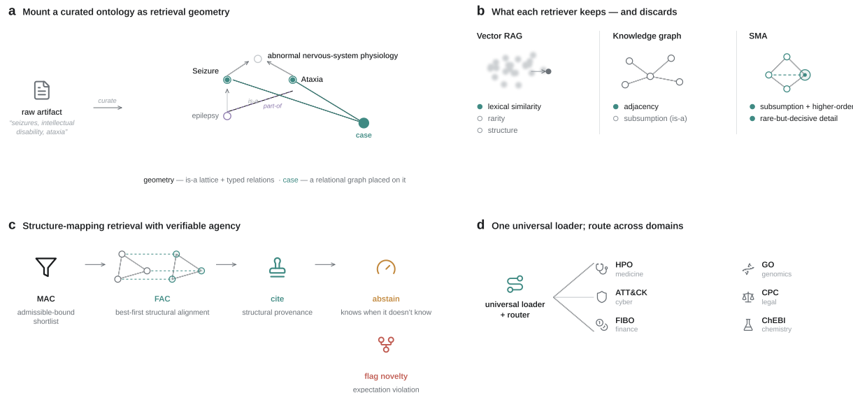
Fig. 1 | A structure-mapping memory grounded in a curated ontology turns a generalist LLM into a verifiable specialist. SMA retrieves on the logical structure that vector RAG and knowledge graphs discard. a, a raw artifact is curated into an expert-maintained ontology — an is-a ascension lattice (geometry) with typed relations — and a case is encoded as functor statements placed on it, so a specific term can match a more general one. b, vector RAG collapses an item to one vector (discarding rarity and structure); a knowledge graph hops by adjacency (no subsumption); SMA keeps subsumption, higher-order structure, and rare-but-decisive detail. c, retrieval is a structural alignment: MAC returns an admissible-bound shortlist, FAC performs best-first structural alignment, and every hit yields a structural citation, with calibrated abstention and novelty flagging. d, one universal loader mounts any open ontology and a router selects the domain per query (HPO, GO, ATT&CK, CPC, FIBO, ChEBI).
