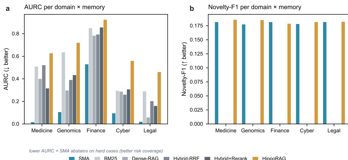
Extended Data Fig. 1 | Per-domain AURC and Novelty-F1 across all six memory systems. a , AURC (area under the risk-coverage curve; lower is better): SMA achieves the lowest AURC in all 5 of 5 domains, indicating superior selective abstention — it correctly withholds on hard or novel queries. Finance is the hardest domain for all methods (sparse ontology coverage). b , Novelty-F1: only SMA and HippoRAG return non-zero novelty-F1; the four lexical/dense baselines cannot distinguish known from unknown at all (novelty-F1 = 0). SMA novelty-F1 ranges from 0.177 (Genomics) to 0.182 (Medicine, Finance, Legal), reflecting the fixed 36-novel-query injection across arms. Source: reports/confirmatory/agentnic_{domain}.csv.
