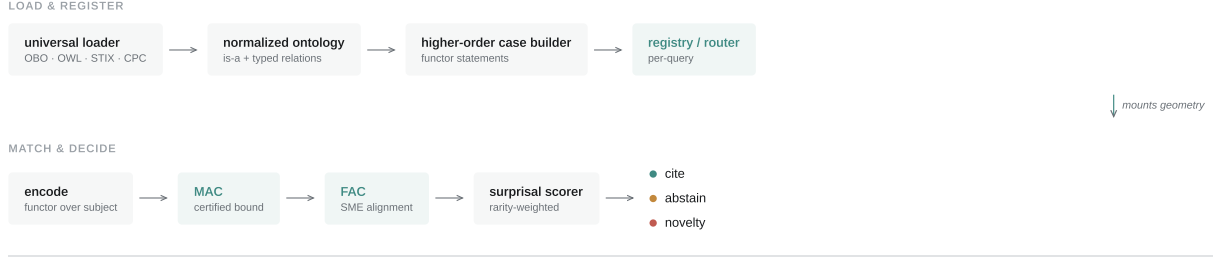
Fig. M | SMA-1 mounts any open ontology, then matches and decides by structural alignment. Load & register , a universal loader ingests open ontology formats (OBO, OWL, STIX, CPC), normalizes them into an is-a + typed-relation geometry, builds higher-order cases as functor statements, and registers them behind a per-query router. Match & decide , a query is encoded as a functor over its subject; MAC returns a certified admissible-bound shortlist, FAC performs structure-mapping (SME) alignment, and a rarity-weighted surprisal scorer routes the result to cite, abstain, or novelty.
