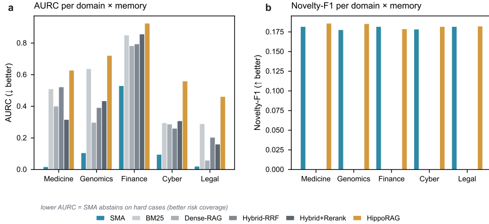
Extended Data Fig. 1 | Per-domain AUC and Novelty-F1 across all six memory systems. a , AUC (area under the risk-coverage curve; lower is better): SMA achieves the lowest AUC in all 5 of 5 domains, indicating superior selective abstention — it correctly withholds on hard or novel queries. Finance is the hardest domain for all methods (sparse ontology coverage). b , Novelty-F1: only SMA and HippoRAG return non-zero novelty-F1; the four lexical/dense baselines cannot distinguish known from unknown at all (novelty-F1 = 0). SMA novelty-F1 ranges from 0.177 (Genomics) to 0.182 (Medicine, Finance, Legal), reflecting the fixed 36-novel-query injection across arms.
