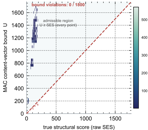
Lemma 2: the screening bound is admissible
