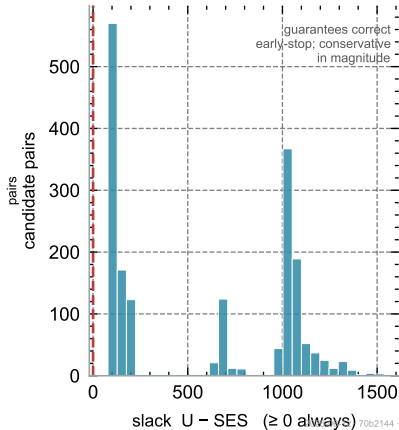
Bound never underestimates the true score
