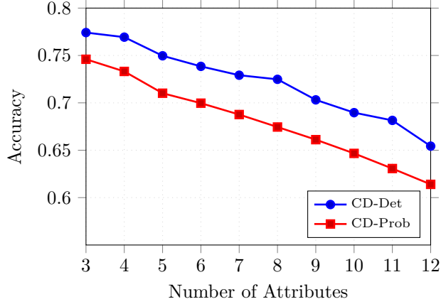
Figure 2: Accuracy versus number of attributes for 10 training samples under class assignment function Y_2
