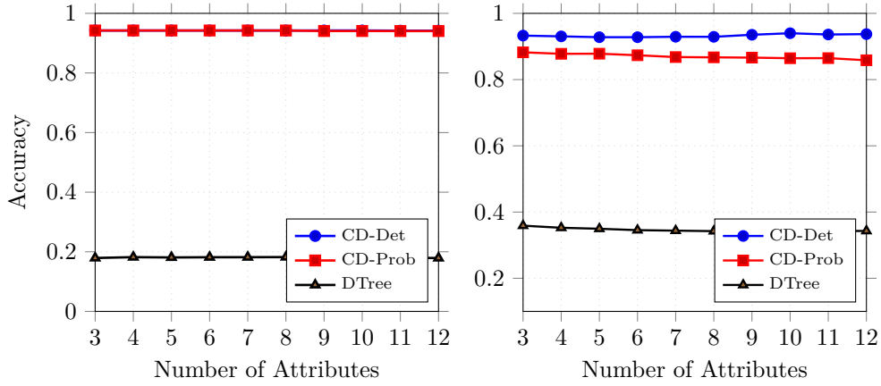
Figure 1: Accuracy versus number of attributes for 20 training samples. Left: under class assignment function Y_1 . Right: under class assignment function Y_2 .
