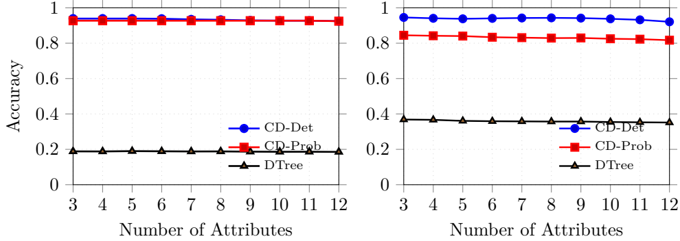
Figure 1: Accuracy versus number of attributes for 20 training samples. Left: under class assignment function Y_1 . Right: under class assignment function Y_2 .
