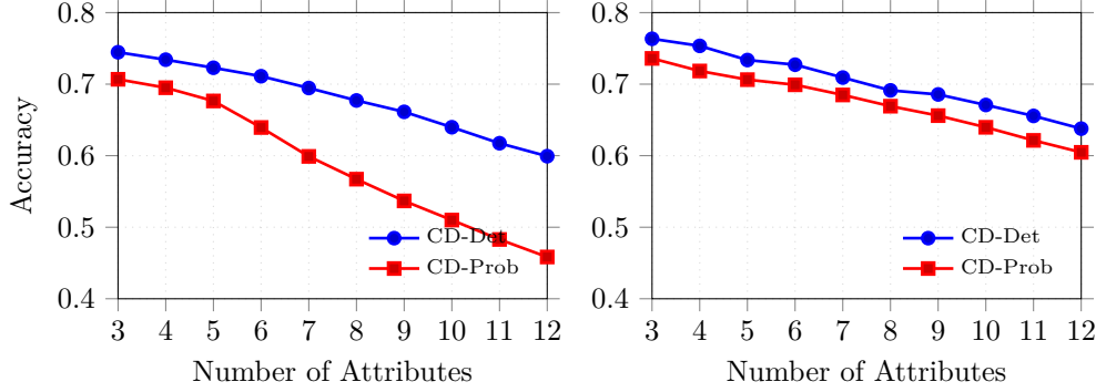
Figure 2: Accuracy versus number of attributes for 10 training samples. Left: under class assignment function Y_1 . Right: under class assignment function Y_2 .
