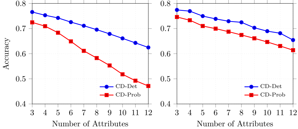
Figure 2: Accuracy versus number of attributes for 10 training samples. Left: under class assignment function Y_1 . Right: under class assignment function Y_2 .
