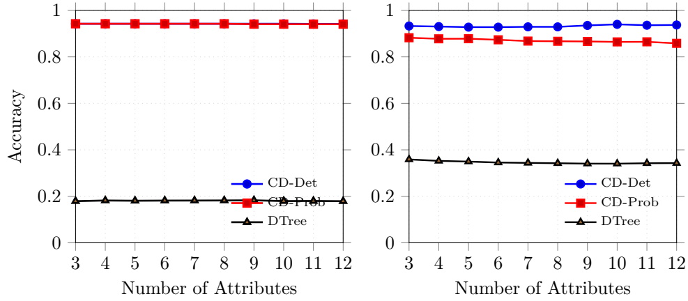
Figure 1: Accuracy versus number of attributes for 20 training samples. Left: under class assignment function Y_1 . Right: under class assignment function Y_2 .
