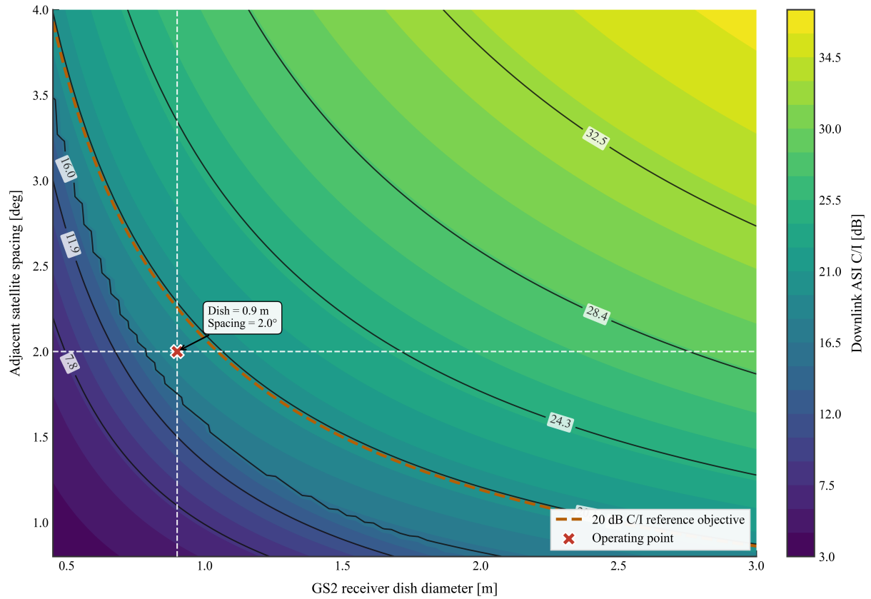
Figure 16: Downlink ASI C/I as a function of orbital spacing and receive-dish diameter.
