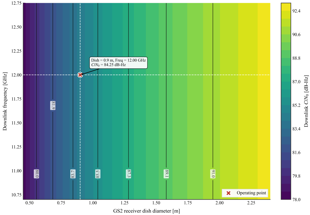
Figure 11: Downlink C/N_0 vs. GS2 dish diameter and frequency.
