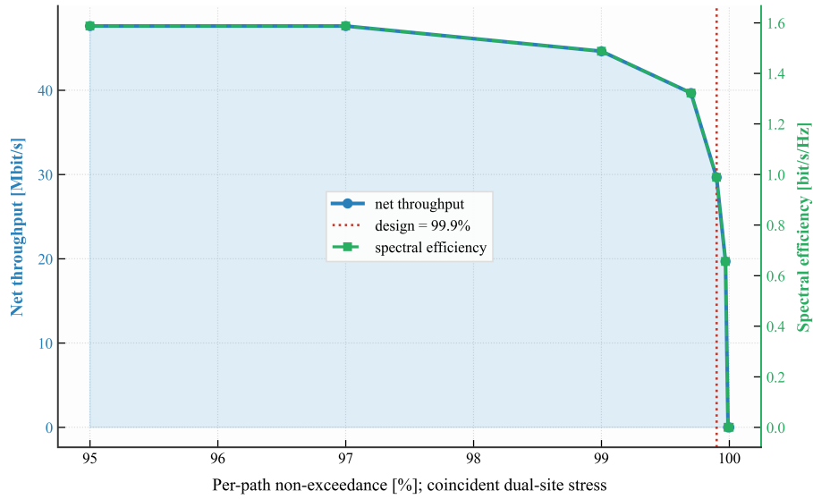
Figure 10: DVB-S2 ACM response over the coincident dual-site per-path exceedance sweep.
