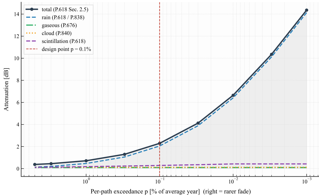
Figure 6: ITU-R slant-path attenuation versus per-path exceedance percentage for the Rome uplink and Ankara downlink.
