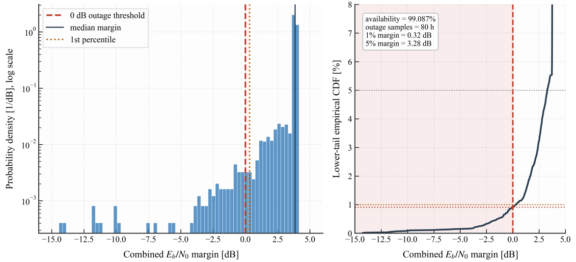
Figure 8: Monte Carlo annual margin distribution and outage-tail summary over 8,760 simulated hourly samples. The left panel shows the log-scale probability density of the combined margin, including the outage threshold, median, and first-percentile markers. The right panel shows the lower-tail empirical CDF, with the shaded region indicating negative-margin samples.
