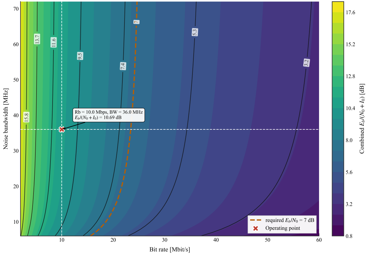
Figure 14: Effective end-to-end E_b/(N_0 + I_0) vs. information bit rate and bandwidth.
