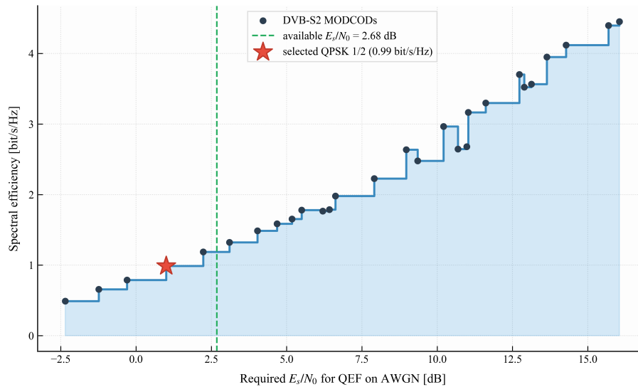
Figure 9: DVB-S2 MODCOD ladder: trade-off between spectral efficiency and required signal-to-noise ratio.
