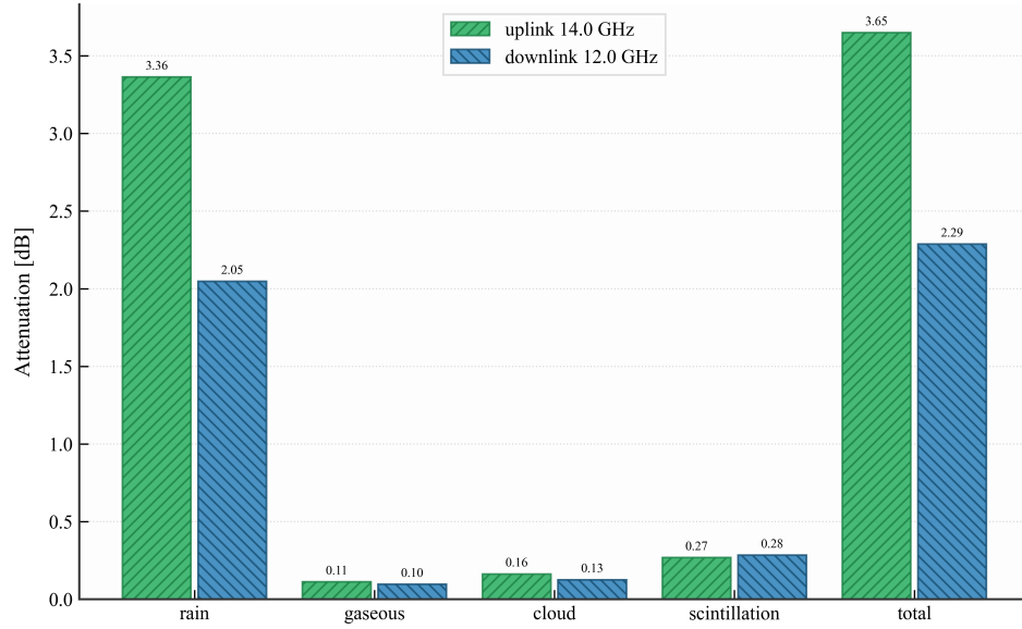
Figure 7: Atmospheric attenuation contribution breakdown at the per-path p = 0.1\% design point.
