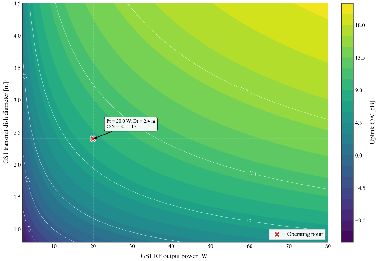
Figure 12: Uplink \frac{C}{N} vs. HPA power and GS1 dish diameter.
