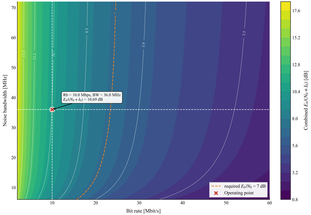
Figure 13: Effective end-to-end \frac{E_b}{N_0 + I_0} vs. information bit rate and bandwidth.
