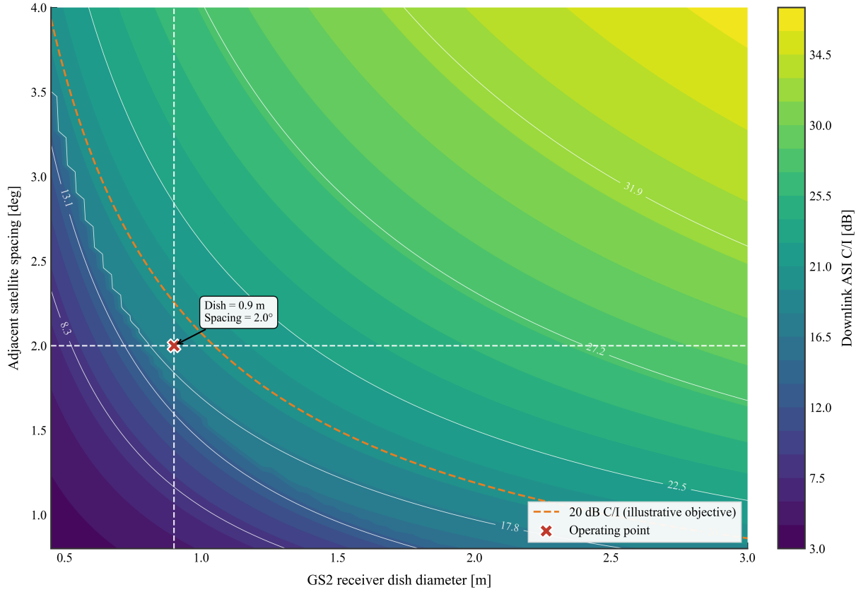
Figure 15: Downlink ASI \frac{C}{I} as a function of orbital spacing and receive-dish diameter.
