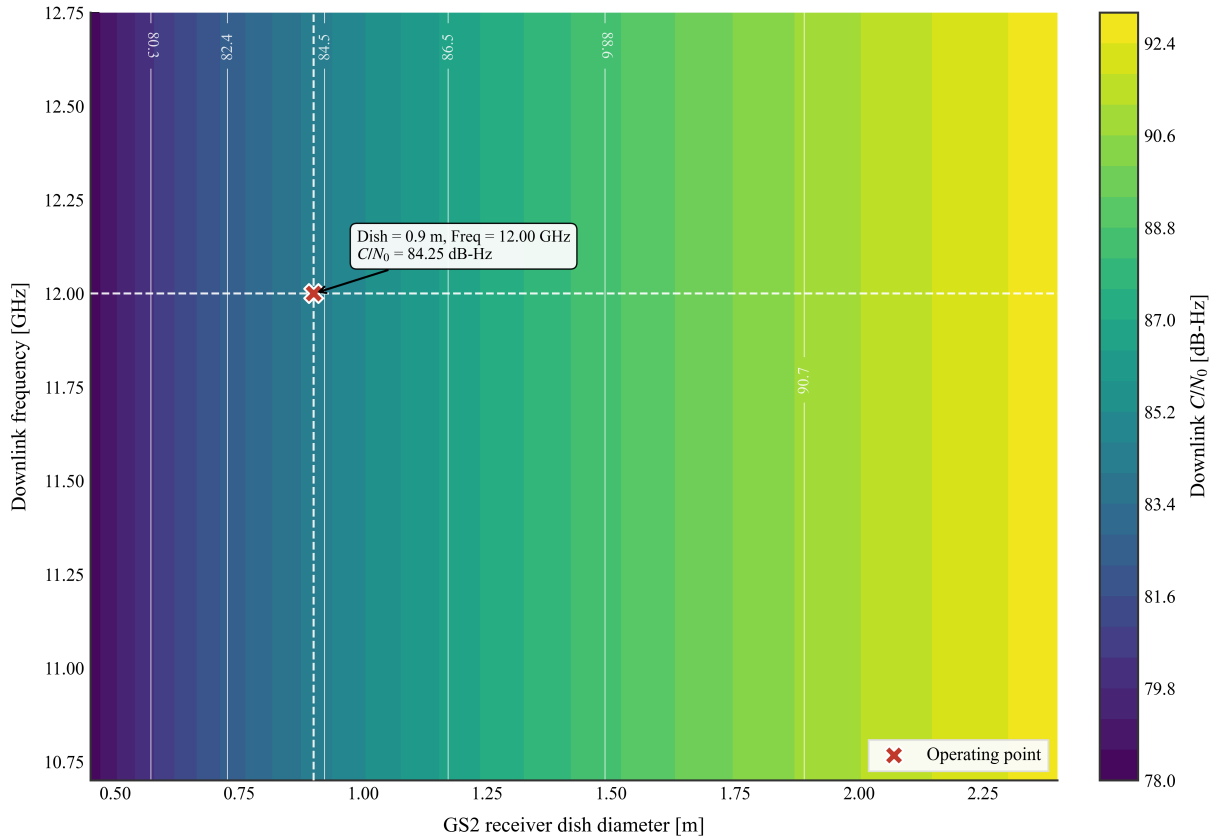
Figure 10: Downlink \frac{C}{N_0} vs. GS2 dish diameter and frequency.
