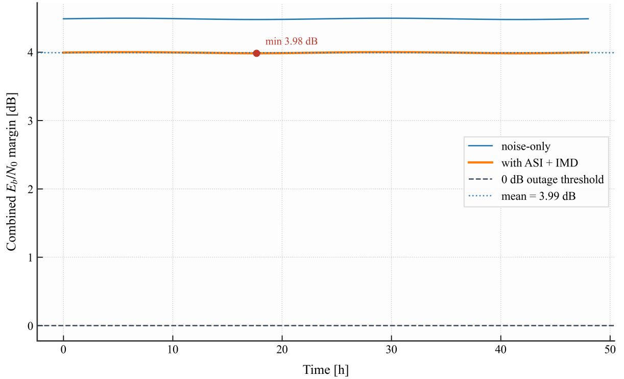
Figure 16: Combined link margin under the modeled apparent GEO motion.
