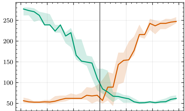
apolune start
