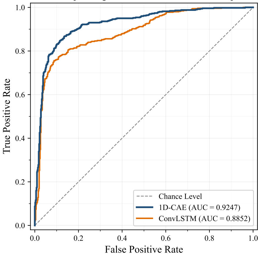
Receiver Operating Characteristic — Model Comparison
