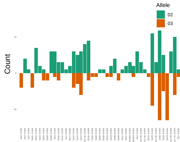
Sequence Count by IGHJ6 allele usage
