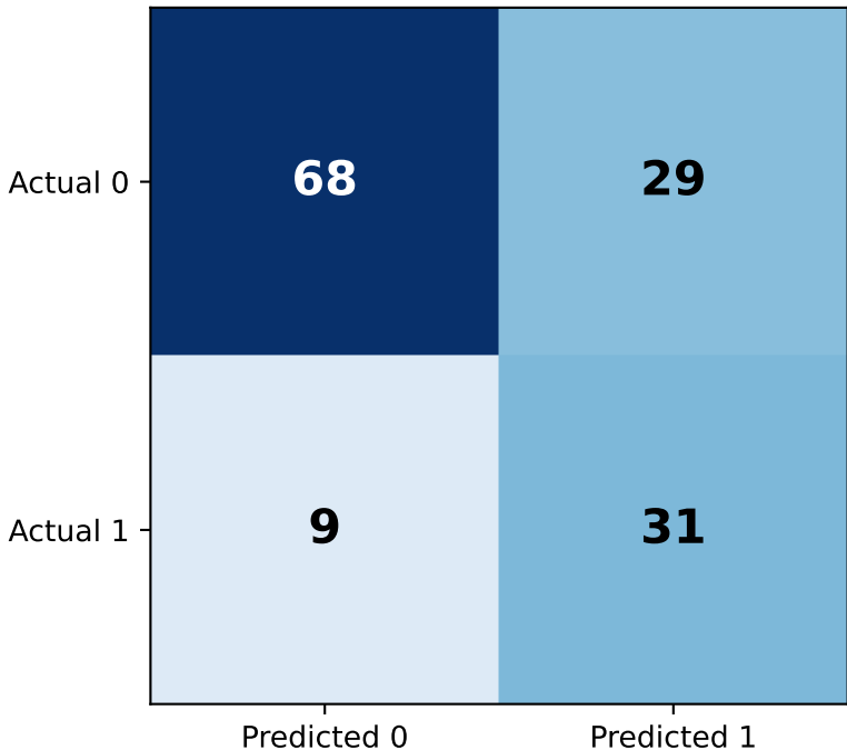
Temporal test-set confusion matrix (n=137)
