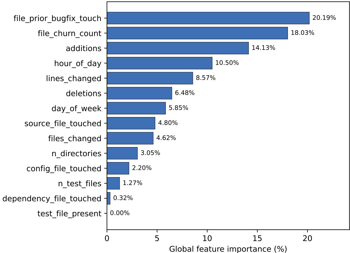
Gradient Boosting feature importances (temporal model)
