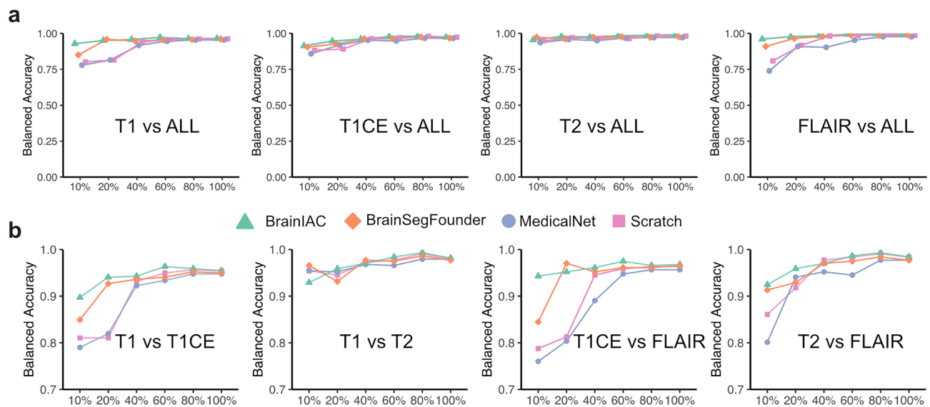
Extended Data Fig. 3 | Sequence classification subgroup analysis. Performance comparison of four models, BrainIAC, BrainSegFounder, MedicalNet, and Scratch, on MRI sequence classification tasks across varying training data sizes (10-100% of available data). a One-versus-all classification performance for
