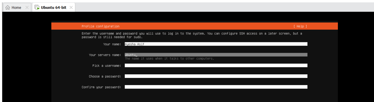
Figure 13.3: ubuntu_username.png
