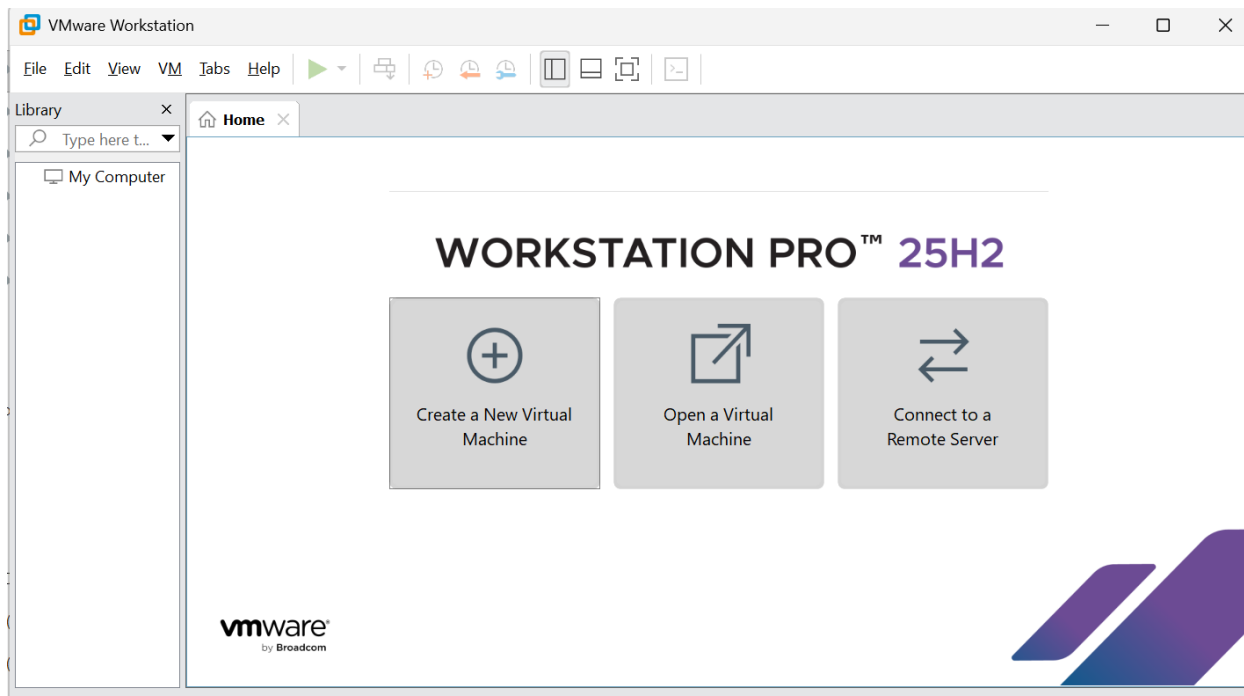
Figure 4.1: vm_creation_wizard.png
