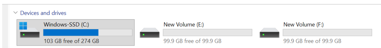
Figure 3.3: available_storage.png
