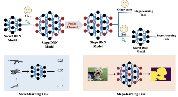
Figure 1: Overview of the proposed deep network steganography framework [3].
