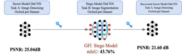
Figure 3: Inter-task deep network steganography framework.
