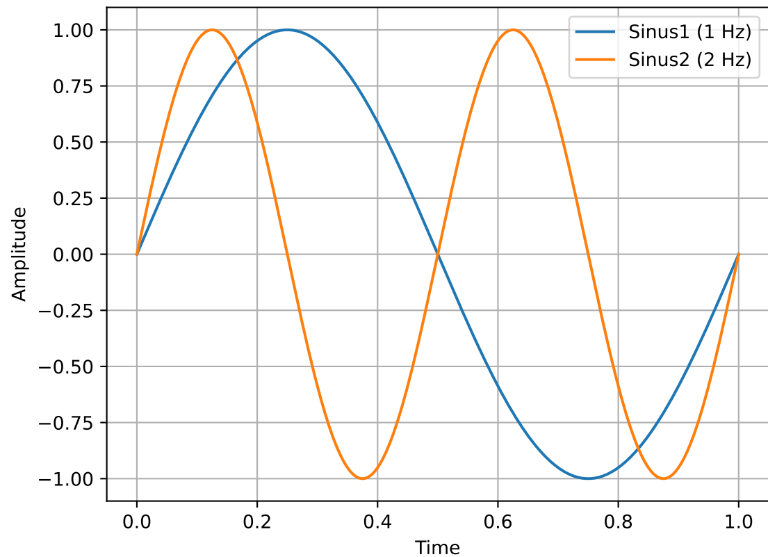
Sinusoidal Functions
