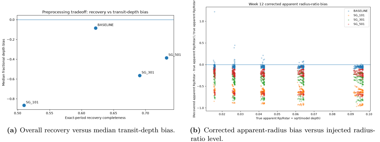
Figure 3: Preprocessing bias. Longer Savitzky–Golay windows improve period recovery in this benchmark but continue to suppress measured depth and the depth-derived apparent radius.
