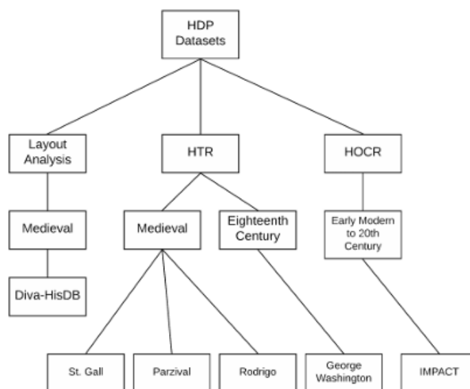
Fig 8. A Hierarchy of HDP Datasets Based on use case and time-period 10
